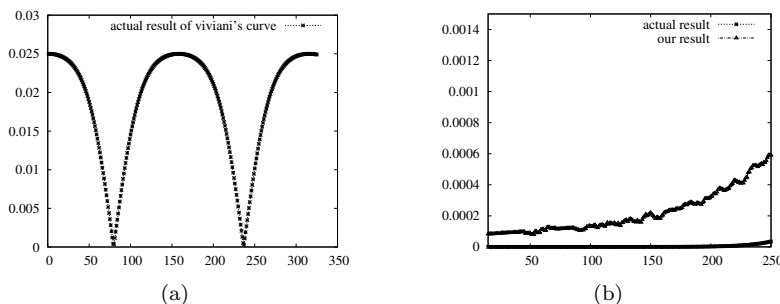
Fig. 9. a: Torsion of Viviani's curve; b: The actual torsion and our result obtained with a hyperhelix curve between the index 15 and 250.
