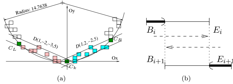
Fig. 2. a. Estimation of the 2D curvature at the point C_k with width 2; b. E_i ( B_{i+1} ) is front (back) of points in first (second) bold edge.
