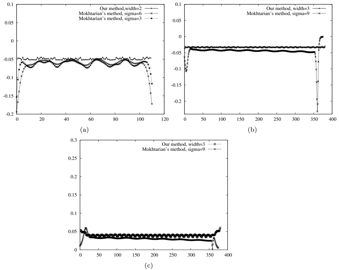
Fig. 11. a. Comparison between our 2D curvature estimator and Mokhtarian's 2D curvature estimator on a circle, radius is 20; b (resp. c): Comparison between our 3D curvature (resp. torsion) estimators and Mokhtarian's 3D curvature (resp. torsion) estimators on an helix curve.
