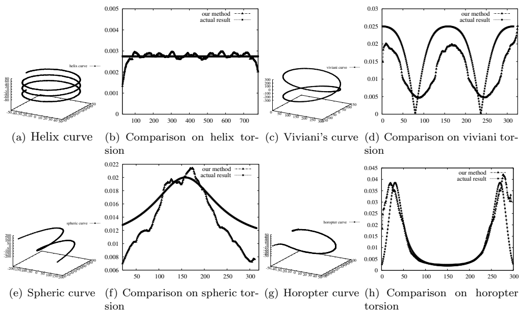
Fig. 7. Experiments on torsion estimator, working width \nu=2 .
