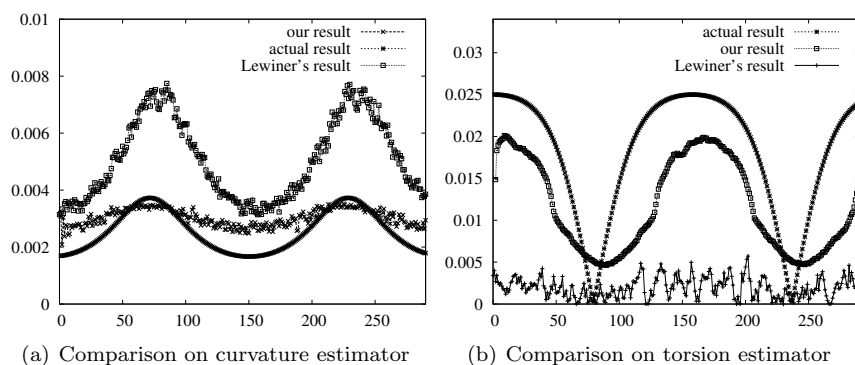
Fig. 10. Comparisons between our curvature and torsion estimators with Lewiner's approach on Viviani's curve. The results of Lewiner are supplied by the author.
