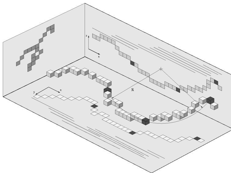
Fig. 3. Given a spatial curve, firstly the set of maximal blurred segments is computed. To determine the curvature value at the second black point, its left (resp. right) extremity is located as the left (resp. right) extremity of the corresponding maximal blurred segment, and then the curvature value is estimated as the inverse of circumcircle radius. Working width is 2.
