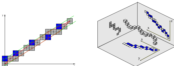
Fig. 1. From left to right: a. \mathcal{D}(5, 8, -8, 11) , optimal bounding line (vertical distance = \frac{10}{8} = 1.25 ) of the sequence of gray points - b. \mathcal{D}_{3D}(45, 27, 20, -45, -81, 90, 90) optimal discrete line of the grey points.
