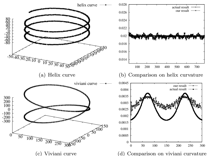
Fig. 6. Experiments of curvature estimator, working width \nu = 2
