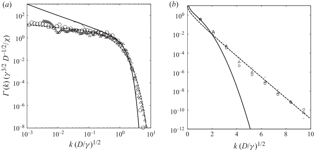
FIGURE 13. Energy spectrum of the scalar at t=7 obtained by direct integration along the strip. The Péclet number is equal to Pe = 10^3 ( \bullet ), Pe = 10^5 ( \Delta ) and Pe = 10^7 ( \circ ). The solid line corresponds to the Batchelor spectrum (5.5) and the dashed line corresponds to the solution (5.9) proposed by Kalda (2000) for decaying turbulence. The scale for the wavenumber is (a) logarithmic and (b) linear.
