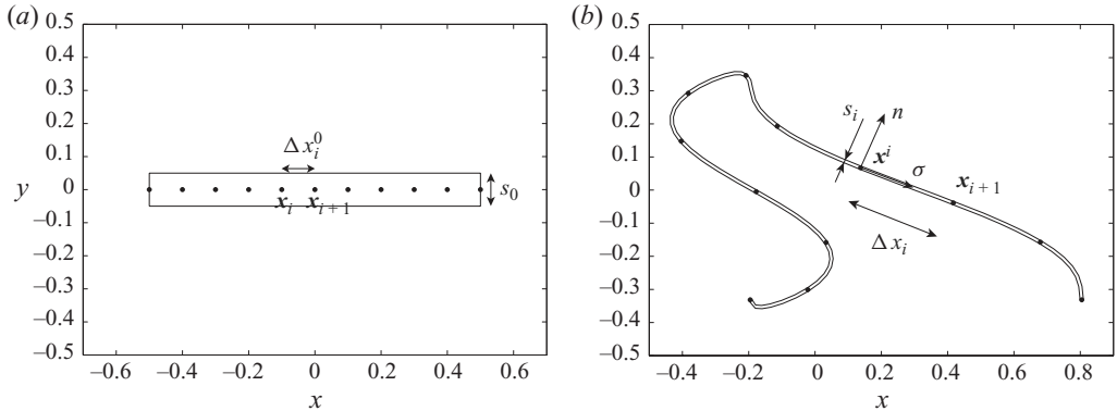
FIGURE 1. Schematic drawing of the evolution of a strip defined by the points \mathbf{x}_i and a striation thickness s_i initially equal to s_0 .
