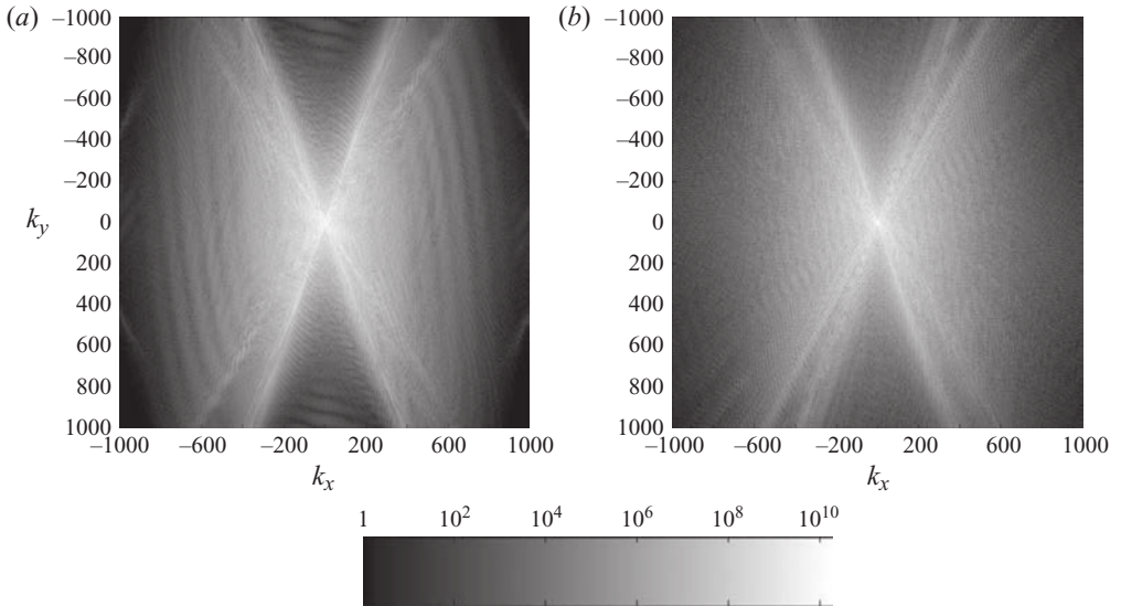
FIGURE 10. Two-dimensional energy spectrum \Phi(\mathbf{k}) of the scalar at (a) t=4 and (b) t=7 for Pe = 10^5 . The spectrum is calculated by a two-dimensional FFT of the scalar spatial distribution c(x) . The grey map is logarithmic in order to visualize large wavenumbers (corresponding to very small values of energy).
