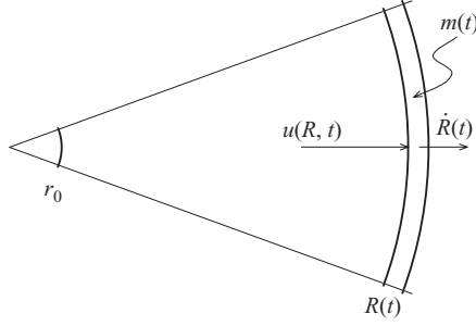
FIGURE 5. Sketch of the rim with mass per unit arclength, m(t) , attached to the sheet with velocity u(R, t) and radius R(t) , used for the mass and momentum balances.
