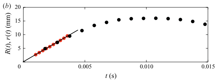
FIGURE 4. (Colour online) (a) Evidence for the radial dependence of the velocity u(r, t) : two initially nearby particles (smoke dust introduced in the liquid prior to drop formation) in the sheet separate along r as time elapses; We = 800 , and time interval between the pictures is 2/3500 s. (b) Time evolutions of the sheet radius R(t) (black dots) and of the position r(t) of a tracer particle in the sheet close to its edge and before it is incorporated in the rim (red dots), recorded simultaneously at We = 10^3 . The black line represents r(t) = u_0 t .
