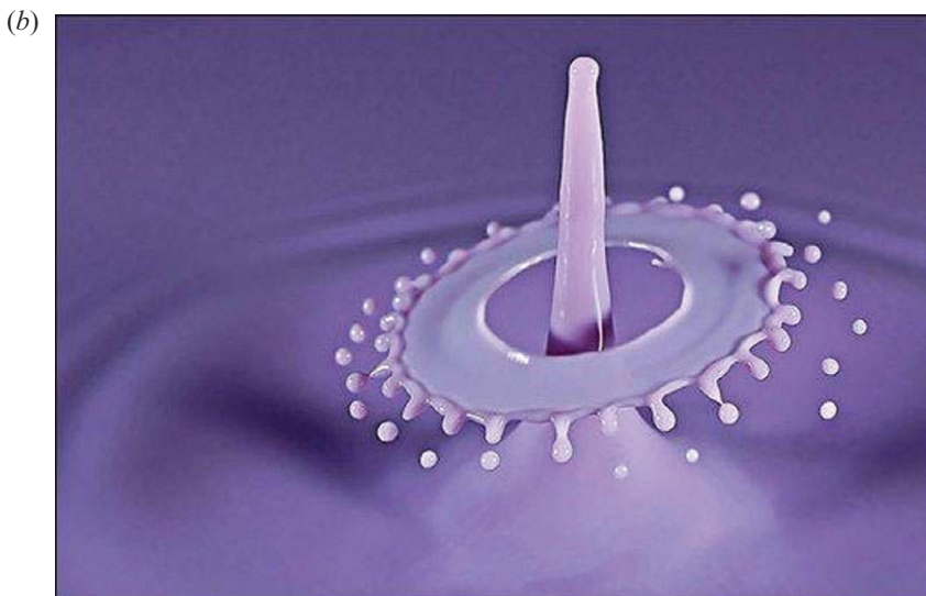
FIGURE 1. (Colour online) (a) Crushing of a water drop falling on a flat dense substrate. Drawing in the margin of folio 33r in the Codex Hammer (previously Codex Leicester, 1506–1510) by Leonardo da Vinci (1508) who notes there the axisymmetry of the impacted drop imprint pattern. Radial fingers are also visible. (b) A dramatic and neat illustration of the phenomenon discussed in the present paper: a train of drops drip into a glass of milkshake; a drop ‘impales’ on the jet emerging from the collapsing cavity formed by the previous drop. The expanding liquid sheet and rim drops are clearly visible. © Irene Müller (2006, http://www.pbase.com/daria90 ), by kind permission.
