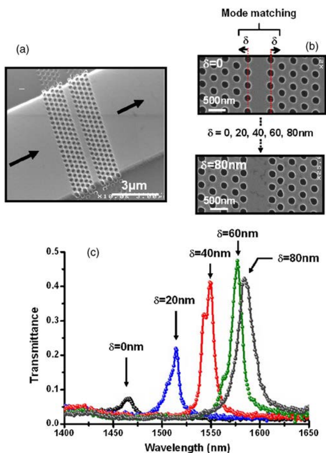
FIG. 1. (Color online) (a) SEM pictures of the investigated microcavities, (b) enlarged view of the cavities with row tuning of \delta=0 and 80 nm, and (c) experimental far-field transmittance spectra of the cavities. The corresponding values of \delta are indicated. The transmittance values are absolute since the presented spectra are normalized by the transmission of an identical waveguide without cavity.
