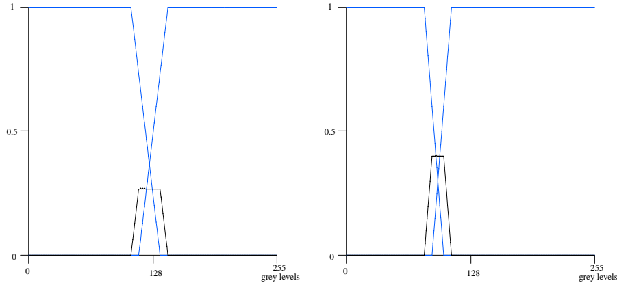
Fig. 24. Eroded mass functions and mass on D for the two images.
