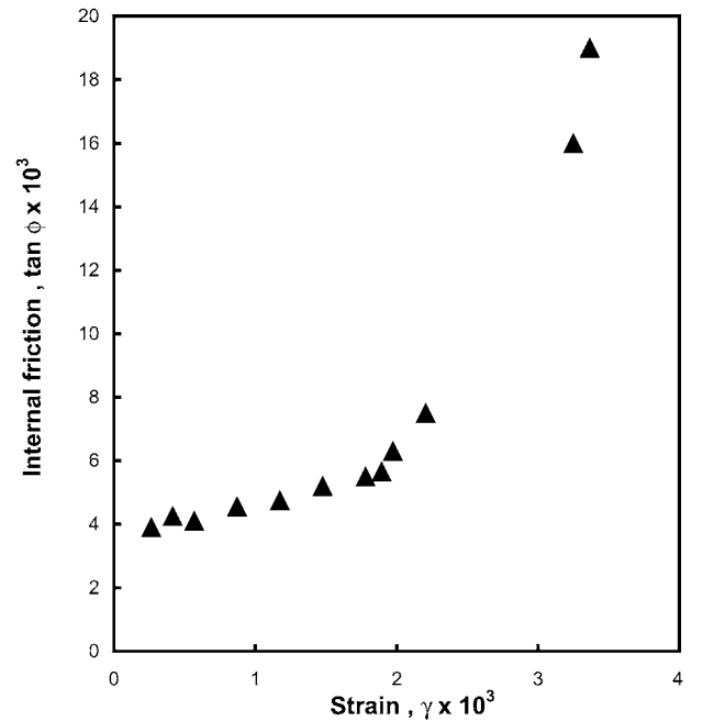
Fig. 2. Internal friction of set plaster, measured on the torsion pendulum at ambient air, vs. strain amplitude.
