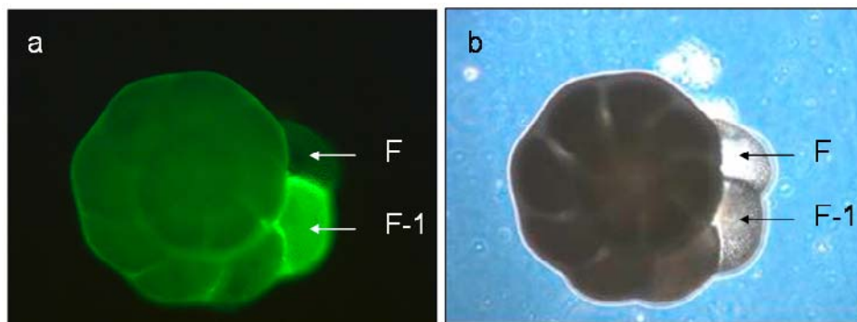
Figure 1. (a) A. tepida specimen showing the calcein labeled penultimate (F-1) and not labeled final (F) chambers under epifluorescent light. (b) Image of the same specimen taken with transmitted light.
