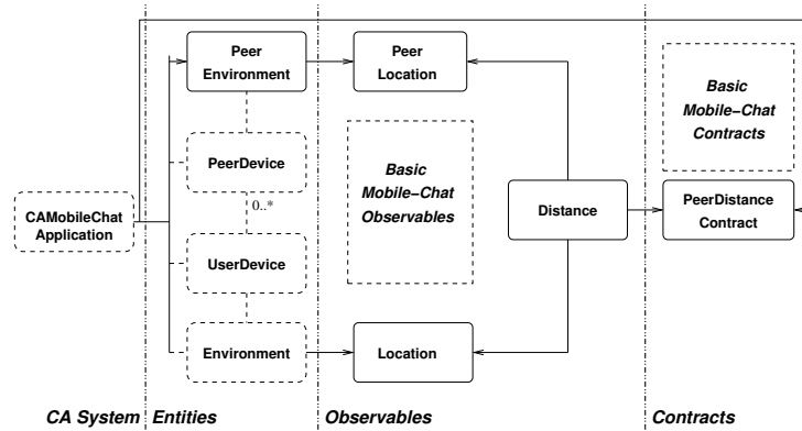
Fig. 5. Model extensions for the plugin location
