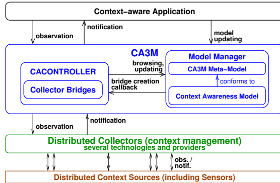
Fig. 2. Runtime architecture of CA3M
