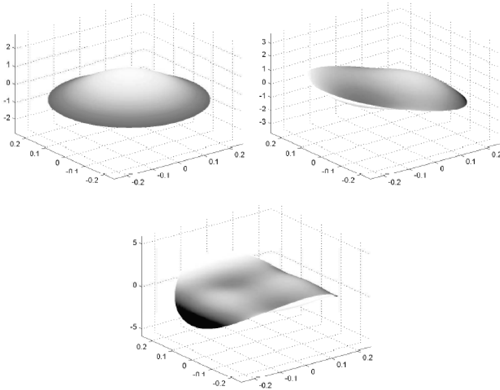
Fig. 6. First three modal deformations of the diaphragm in free-supported conditions.
