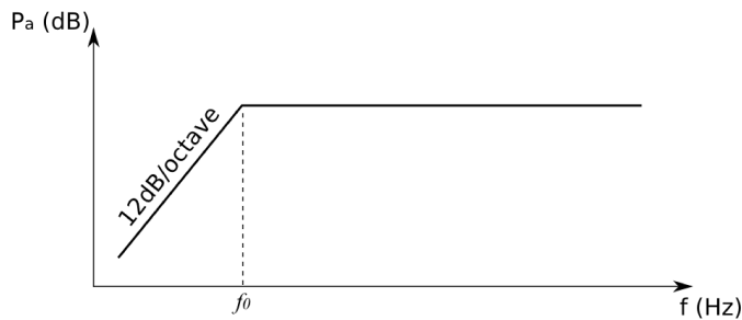
Fig. 2. Behaviour of the pressure response of a loudspeaker vs. frequency.
