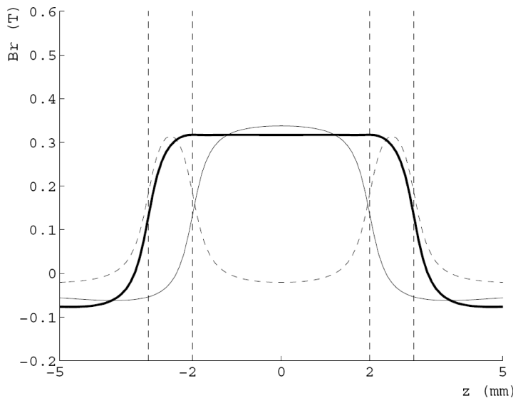
Fig. 3. Radial magnetic induction, B_r (T), created by the three rings structure (bold line), by its central ring (full line) and by its two external rings (dashed line). The vertical dashed lines reflect the heights of the three rings.
