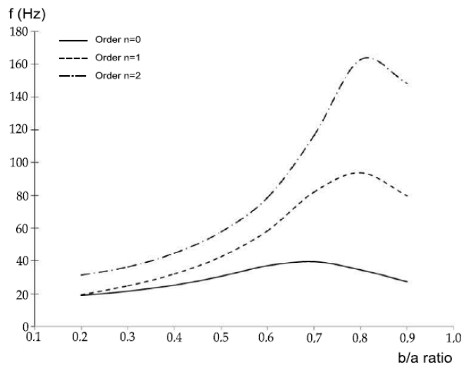
Fig. 5. Evolution of the eigenfrequencies of an arbitrary circular plate (diameter a ), when fixed to a circular support whose diameter b varies.
