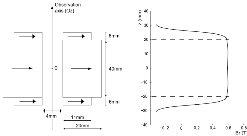
Fig. 4. Magnetic structure used in our first woofer and its created radial magnetic induction, Br (T), along the observation axis.
