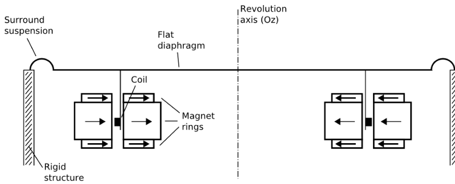
Fig. 1. Composition of the ironless flat loudspeaker.
