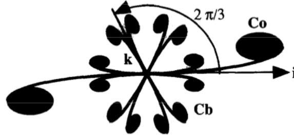
Figure 7: representation of the construction of a trigonal tensor Cb from a triclinic tensor Co .
