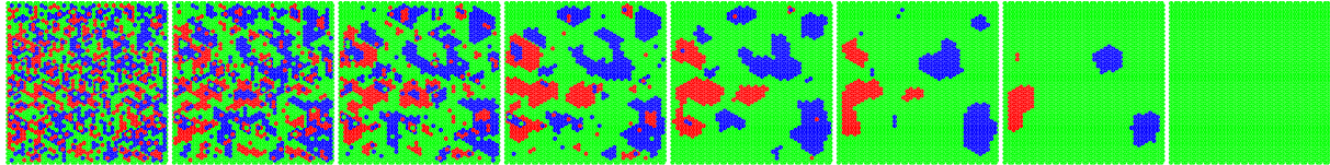
Figure 6. Snapshots (every 600 flips) of the simplified cooling of the same tiling as Fig. 4.
