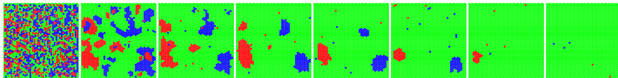
Figure 4. Snapshots (every 1500 flips) of the cooling of a dimer tiling.
