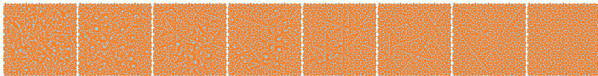
Figure 5. Snapshots (every 5000 flips) of the cooling of a Penrose tiling.
