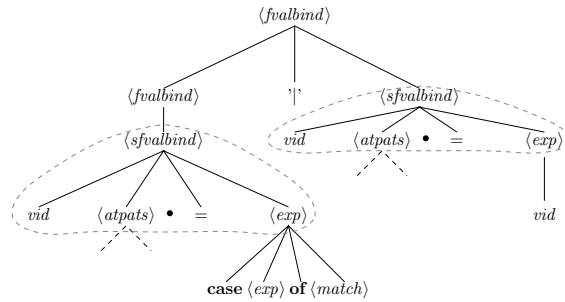
Figure 5: Two equivalent positions under the LR(0) item approximation, corresponding to the single item [\langle sfvalbind \rangle \rightarrow vid \langle atpats \rangle \bullet = \langle exp \rangle] .
