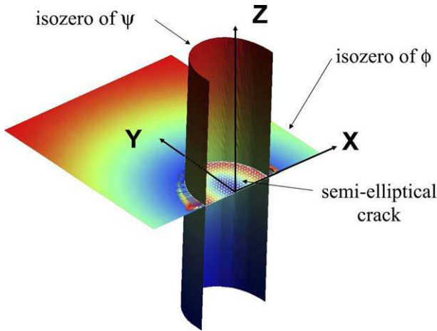
Fig. 4. The surface in the (X-Y) plane is the iso-zero surface of the level set function \phi(x) and represents the crack surface. The “curved” surface normal to the (X-Y) plane is the iso-zero surface of \psi(x) and represents the crack front, which corresponds to the intersection of these two iso-zero surfaces.
