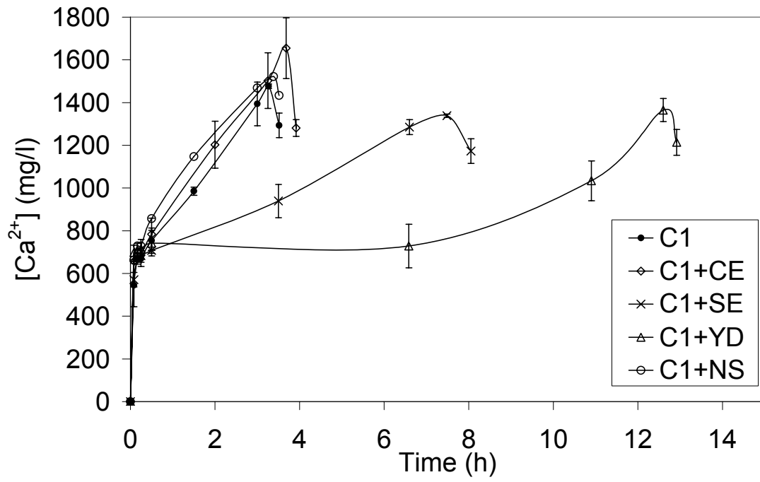
Fig. 7. Evolution of Calcium concentration in admixed suspensions
