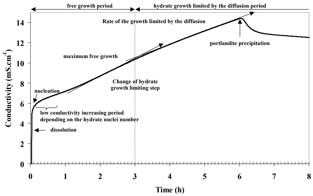
Fig. 2. Different steps of a conductimetric curve
