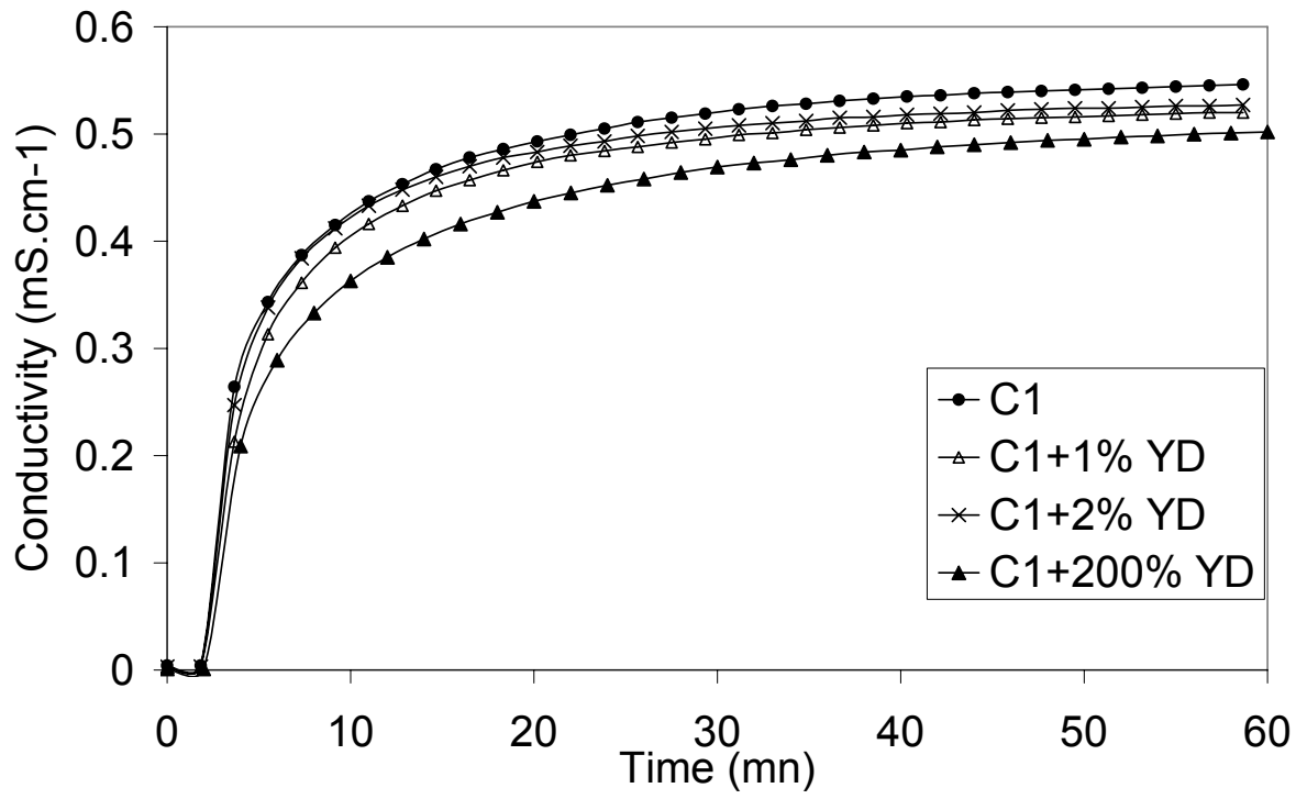
Fig. 6. Effect of YD addition on cement dissolution
