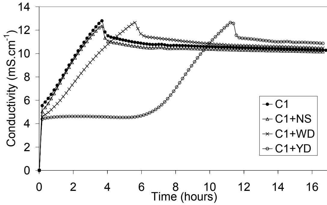
Fig. 5. Effect of dextrinization on the conductimetric curves
