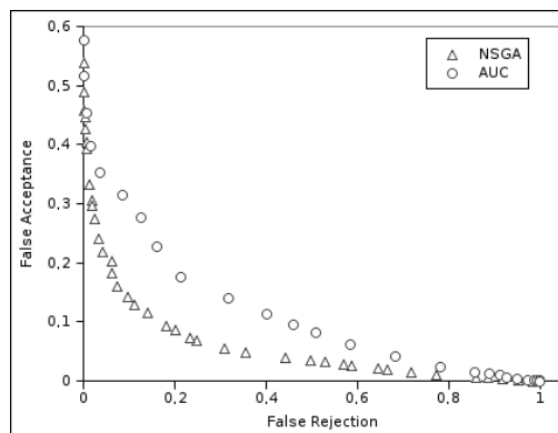
Figure 2. FA/FR curves obtained using NSGA-II and AUC.
