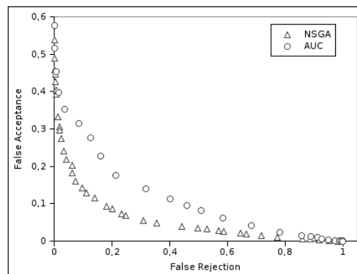
Figure 2. FA/FR curves obtained using NSGA-II and AUC.
