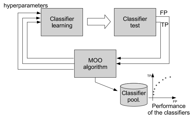
Fig. 1. Multi-model selection framework
