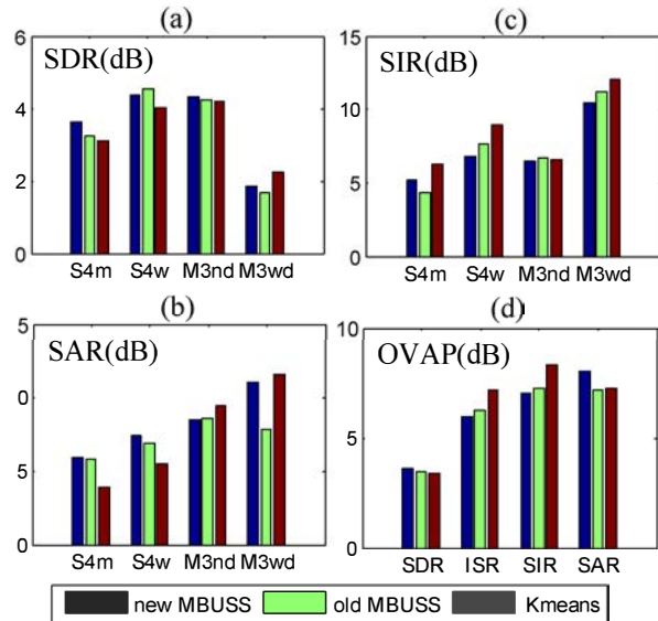
Figure 3: (a),(b),(c) presents respectively the SDR, SAR and SIR performance for each type of mixture; (d) presents the OVAP
