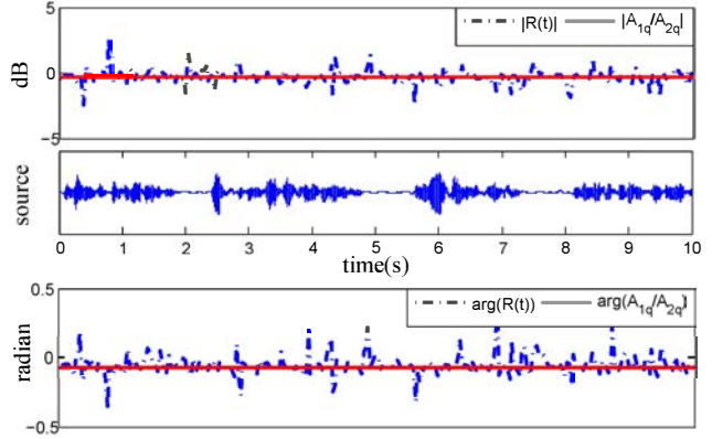
Figure 1: Ideal and observed (IPD, log(ILD)) for a single source mixture at the 100Hz center frequency
