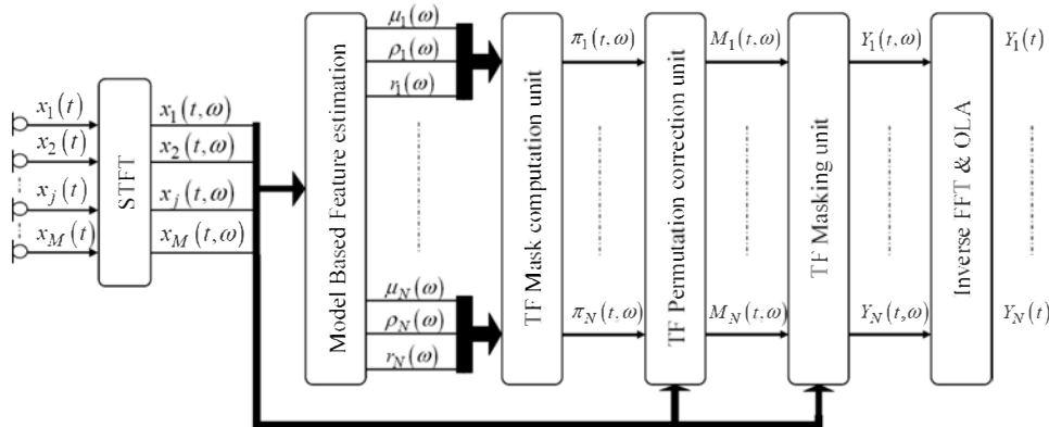
Figure 2: Basic scheme of Model Based Source Separation Approach
