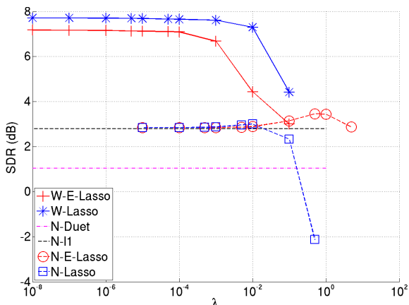
Fig. 1. Variation of the average SDR as a function of \lambda over speech mixtures with N = 4 sources, RT_{60} = 250 ms and d = 1 m.
