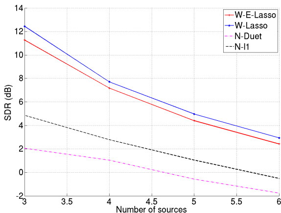
Fig. 2. Variation of the average SDR as a function of N over speech mixtures with RT_{60} = 250 ms and d = 1 m.
