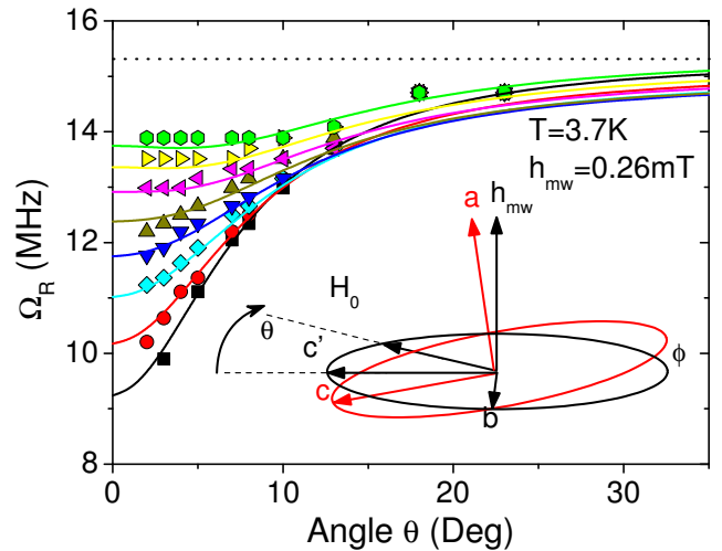
FIG. 3: (color online) Evolution of \Omega_R when the static field H_0 rotates by an angle \theta around the microwave field h_{mw} . Colored continuous lines are computed numerically. Inset: geometry of the experiment where the sample defined by its axes a, b, c is tilted by a small angle \phi \sim 7^\circ around the b=b' -axis. The dotted line represents the conventional equation \Omega_R = g^\alpha \mu_B h_{mw}^\alpha / 2h [21].
