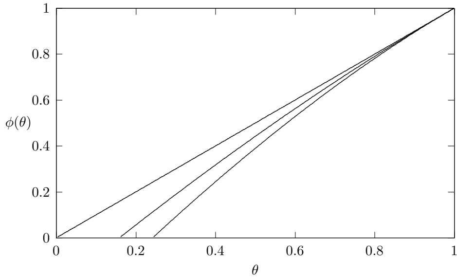
Figure 2: Optimal selectivity function (uniform distribution)
