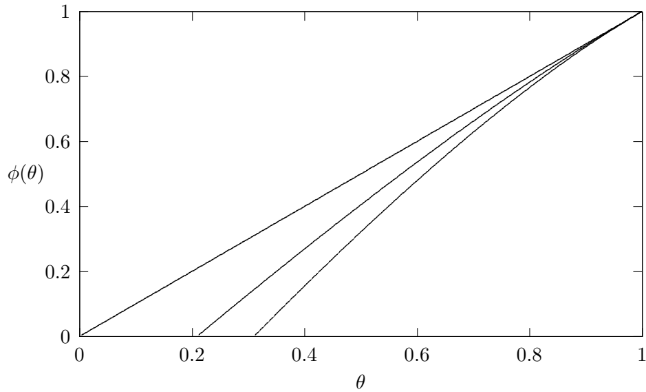
Figure 3: Optimal selectivity function (quadratic distribution)
