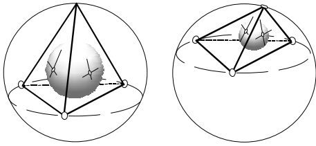
Fig. 2. Representation of circumscribed sphere and insphere
