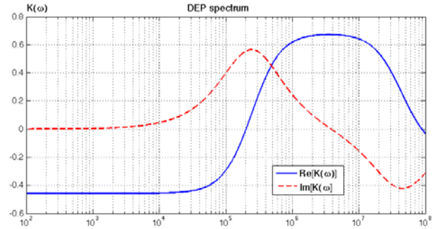
Fig. 9. Theoretical dielectrophoresis spectrum of a Jurkat cell, real and imaginary part. See Table I for the dielectric properties of the cell; \sigma_m = 50 \text{ mS}\cdot\text{m}^{-1} and \epsilon_m = 80 \epsilon_0 for the medium. R = 5 \mu\text{m} , e = 5 \text{ nm} .
