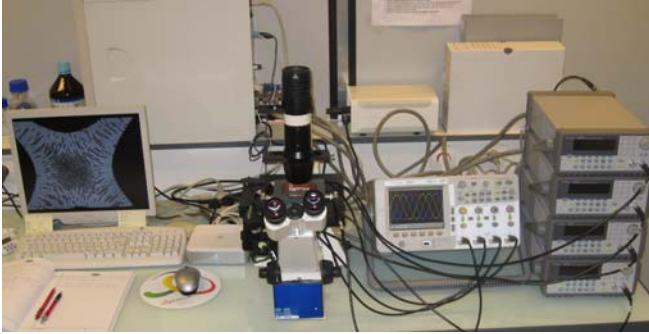
Fig. 11. Platform for dielectrophoretic spectrum acquisition.
