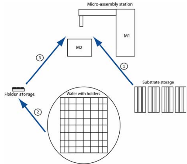
Fig. 8. Description of the general assembly sequence.
