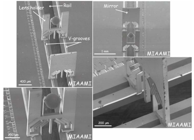
Fig. 11. SEM pictures of the assembled demonstrator.
