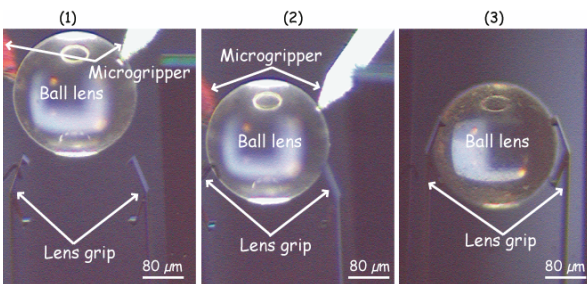
Fig. 10. Assembly sequence of ball lens using a microgripper: (1) the ball lens is gripped by the microgripper and align to the lens grip, (2) the ball lens is inserted to the lens grip, and (3) the ball lens is released and maintained into the lens grip.
