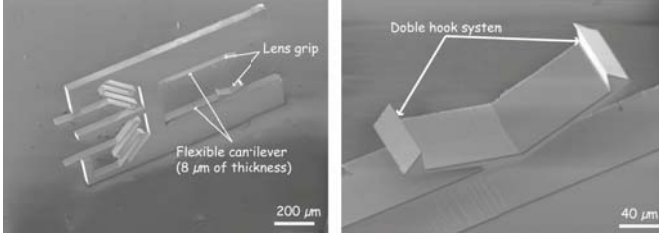
Fig. 5. SEM pictures of the designed lens holder
