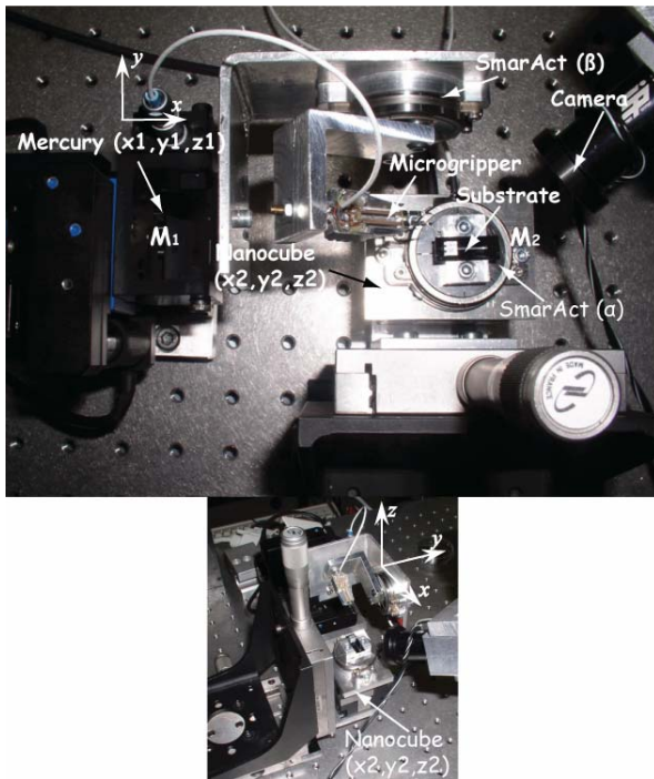
Fig. 7. Developed micro-assembly station for micro-optical benches.
