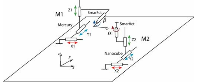
Fig. 6. The kinematic scheme of the microrobotic structure.
