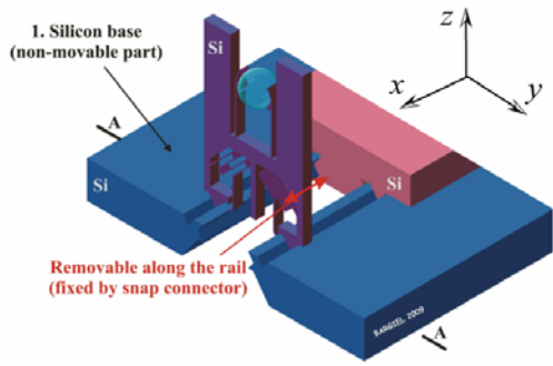
Fig. 1. RFS-MOB concept: general view.
