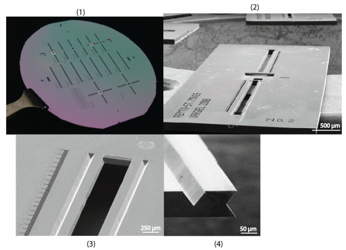
Fig. 4. Microfabricated substrate using DRIE and KOH etching: (1) general view of the wafer, (2) bench with straight rail after dicing, (3) the rail with a ruler, and (4) view of V-groove and the vertical V-groove.
