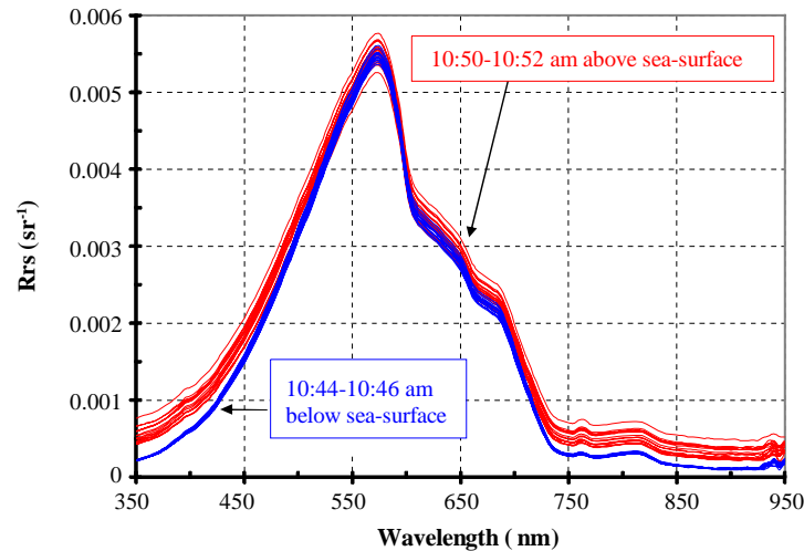
Fig. 8. Remote-sensing reflectance calculated from irradiance and radiance shown in Fig. 5 and 6 at Aiguillon on 17 February 2004: Rrs = Lw/Ed with Lw computed from Lu(-2) in blue (measurements taken between 10:44 am and 10:46 am) and Rrs = L(+2)/Ed in red, measurements taken between 10:50 am and 10:52 am).
