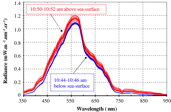
Fig. 6. Upwelling radiance measured at +2\text{cm} \pm 1\text{cm} (17 red curves) and at -2\text{cm} \pm 1\text{cm} (13 blue curves, uncorrected radiance) simultaneously with an irradiance measurement presented in Fig. 5. Aiguillon, 17 February 2004.
