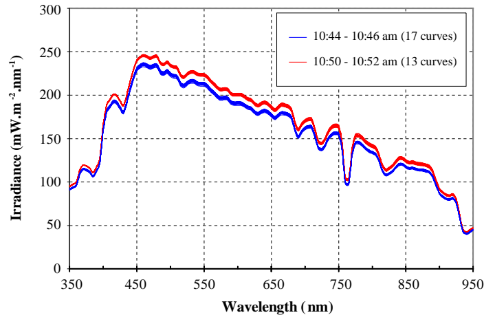
Fig. 5. Irradiance measured at Aiguillon under a covered sky on 17 February 2004 between 10:44 and 10:46 am and between 10:50 and 10:52 am.
