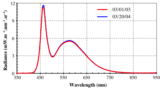
Fig. 1. Calibration radiance spectra measured using the FieldCal device.
