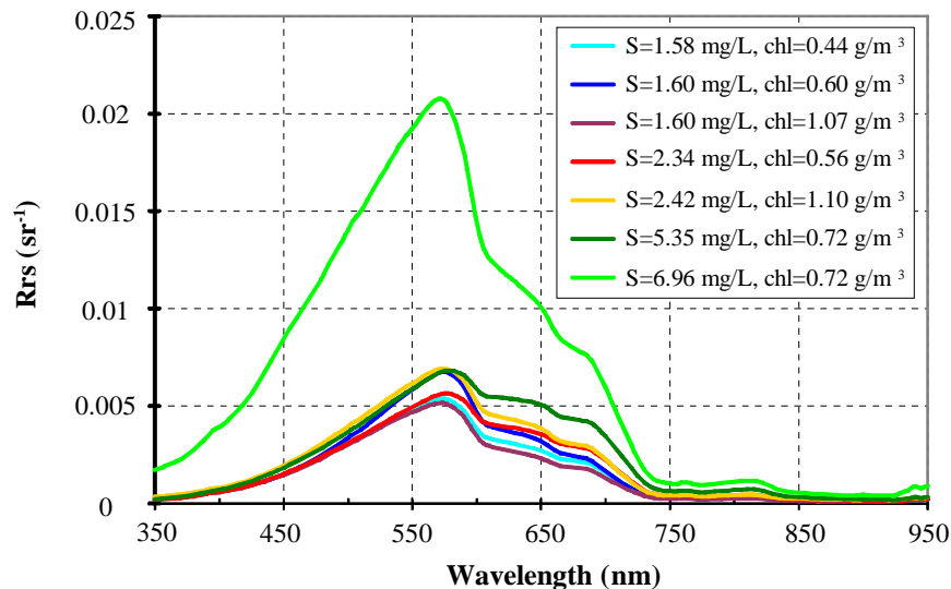
Fig. 9. Remote-sensing reflectance and corresponding concentrations in Total Suspended Matter (S) and in chlorophyll-a (chl) for 7 stations in the Bay of Arcachon, 17 and 18 February 2004.
