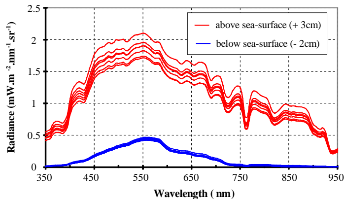
Fig. 7. Radiance measured above-water at +3\text{cm} (7 red curves) and below the sea surface at -2\text{cm} (33 blue curves, uncorrected measurements), Teychan, 18 February 2004.
