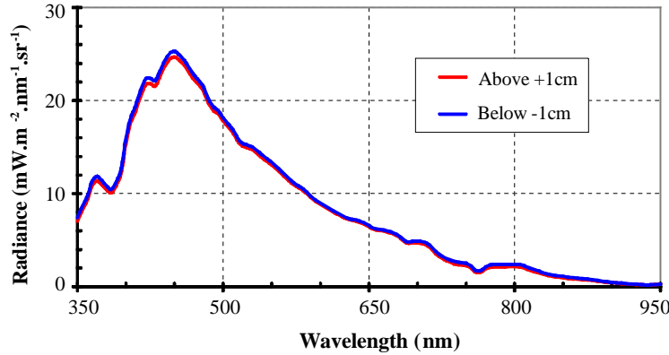
Fig. 4. Spectral radiances obtained following the schema of Fig. 3. The below-water spectrum L(\lambda, -1) corresponds to a non-corrected radiance.
