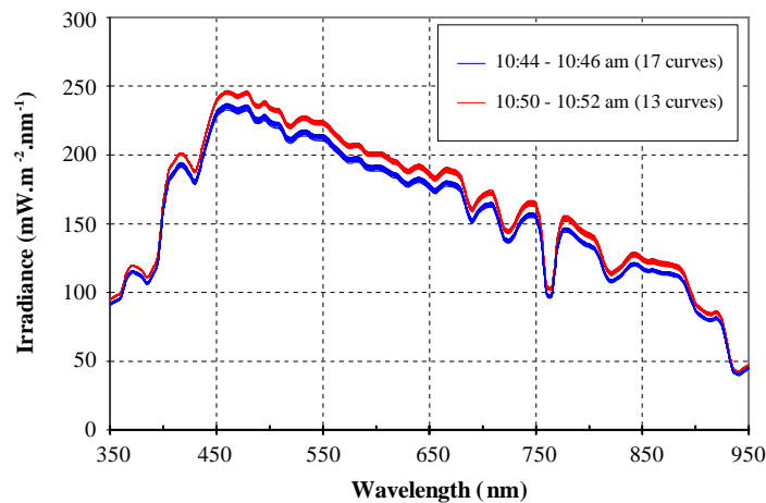
Fig. 5. Irradiance measured at Aiguillon under a covered sky on 17 February 2004 between 10:44 and 10:46 am and between 10:50 and 10:52 am.
