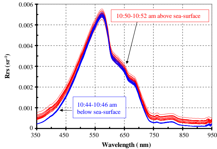
Fig. 8. Remote-sensing reflectance calculated from irradiance and radiance shown in Fig. 5 and 6 at Aiguillon on 17 February 2004: Rrs = Lw/Ed with Lw computed from Lu(-2) in blue (measurements taken between 10:44 am and 10:46 am) and Rrs = L(+2)/Ed in red, measurements taken between 10:50 am and 10:52 am).
