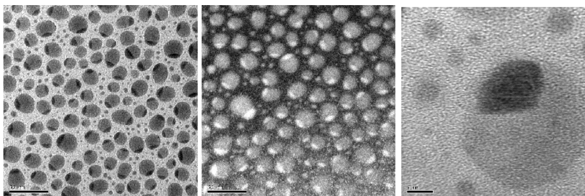
Figure 2: Left: bright field TEM image of a Ga-Pb sample at T=202°C. Center: dark field TEM image
