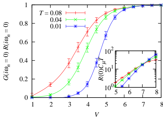
FIG. 4: (color online) Product G(i\omega_n = 0)R(i\omega_n = 0) for K = 1/3 as a function of the backscattering strength V , for different temperatures T . For D and \Delta/(2K^2) , we use the same parameters as in Fig. 2. Inset: R(0)C_\mu T as a function of V , for different T ; the crossing of the curves gives a good estimate of the transition point.
