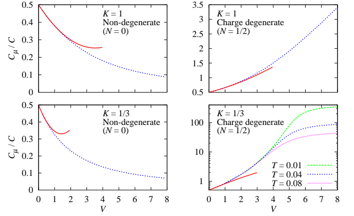
FIG. 2: (color online) Capacitance C_\mu as a function of the backscattering strength V , obtained at temperature T = 0.04 with Monte Carlo computations (dashed lines). The solid lines show the predictions of the perturbative calculations up to second order. We take E_C/\pi^2 as the unit of energy and use the parameters D \equiv 2\pi J/\beta = 8\pi and \Delta/(2K^2) = \pi^2 . Temperature dependence is shown in the bottom right panel, where the vertical axis is measured on a logarithmic scale.
