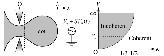
FIG. 1: Left: schematic view of the mesoscopic capacitor: a 1D quantum dot, capacitively coupled to a gate with time-dependent voltage V_g + \delta V_g(t) . Right: schematic phase diagram in the degenerate case. V_c denotes the critical backscattering strength for K = 1/3 .
