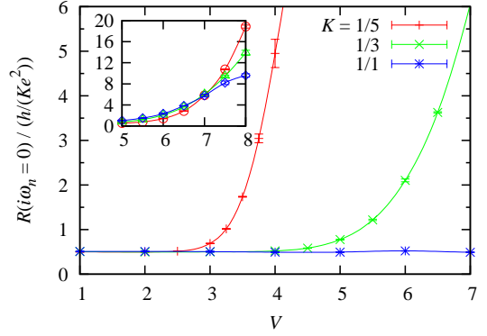
FIG. 3: (color online) Extrapolated value R(i\omega_n \rightarrow 0) as a function of V at temperature T = 0.04 in the degenerate case. For D and \Delta/(2K^2) , we use the same parameters as in Fig. 2. Inset: R(i\omega_n \rightarrow 0) for K = 1/3 at T = 0.01 ( \circ ), 0.04 ( \Delta ) and 0.08 ( \diamond ) in the vicinity of the location where the crossing occurs.
