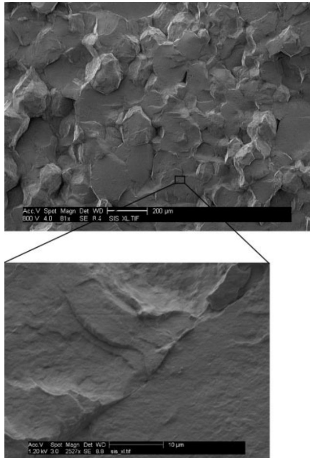
Figure 11 LVSEM room-temperature fracture surface observation: POM-high HVC.
