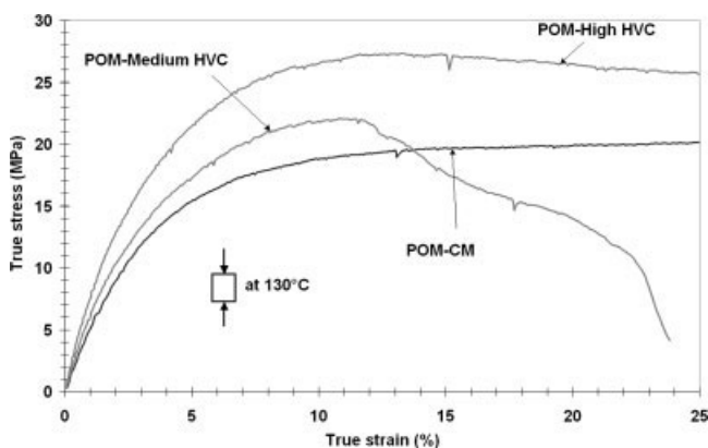
Figure 15 Stress-strain curves from compressive tests at 130°C.
