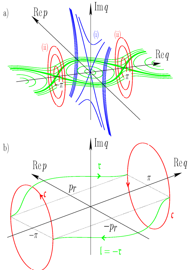
Figure 4: With the choice of a complex-time path given in 3) (one-step path), the contributions to \text{tr}(\tilde{S} \hat{I}_n \hat{U}(T)) come from one half symmetric periodic orbits \circ (b) that are a composite of 1) (repetitions of) a periodic orbit \tau of period T_\tau in the phase-space plane (\text{Re } q, \text{Re } p) at energy E > \gamma (recall that the planes q = \pm\pi are identified); 2) one half of a periodic orbit \circ of period T_\circ in the phase-space plane (\text{Im } q, \text{Re } p) at energy E .
