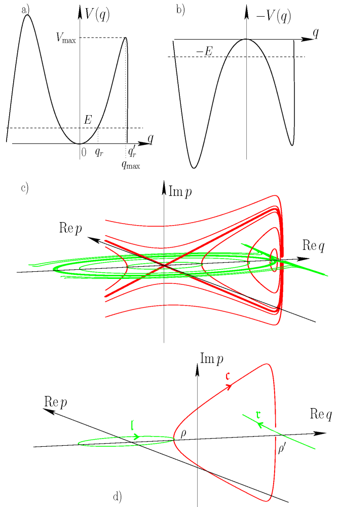
Figure 8: (colour online) The escape rate at energy E from an island created by a confining potential V whose shape is shown in a) can be semiclassically computed in terms of complex classical orbits where one canonical coordinate, say q , is kept real. In phase-space, this trajectory appears to be a concatenation of two types of curves that join on the (\text{Re } q) -axis: 1) a trajectory that lies in the phase-space plane (\text{Re } q, \text{Re } p) with real variations of t at energy E with the potential V and 2) a trajectory that lies in the phase-space plane (\text{Re } q, \text{Im } p) with imaginary variations of t at energy -E with the potential -V shown in b). In c) a family of constant energy curves is shown (horizontal green for the first type, vertical red for the second type). In d) for a given energy, we show how three curves l, c, r glue together at the turning points.
