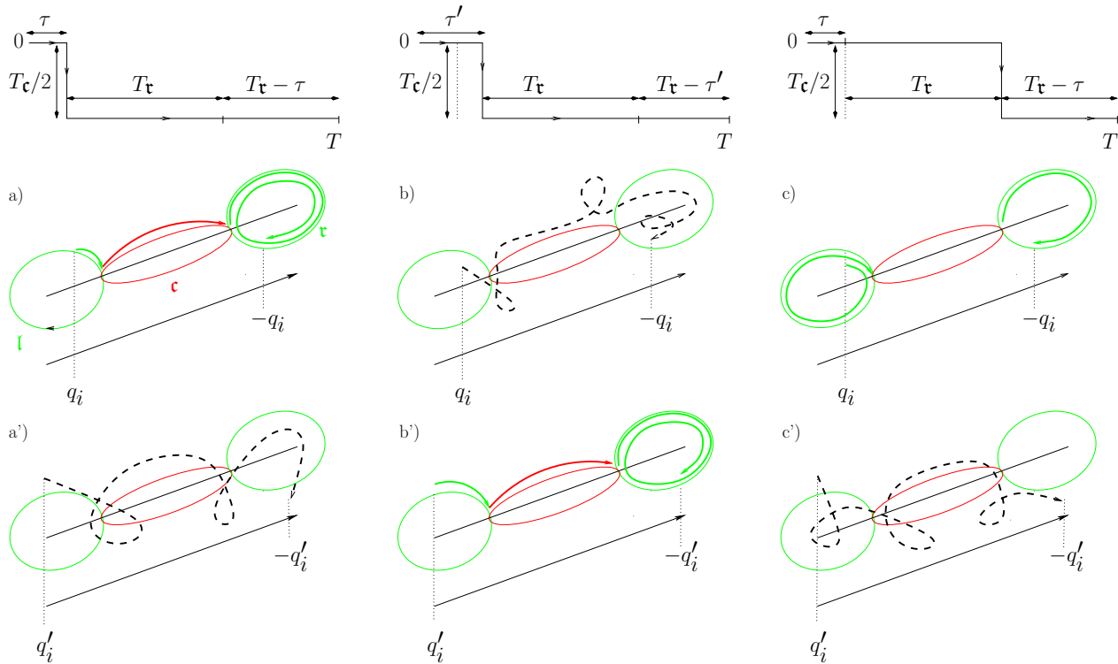
Figure 3: (colour online) For the double well in Fig. 1, at a given energy 0 < E < V_{\max} , when T = 2T_r(E) - iT_c(E)/2 , for each one-step time path, there exists a unique half symmetric periodic orbit with energy E keeping \text{Im } q = 0 starting from the left authorised region. Its initial point is uniquely defined: For the time-path depicted in the left column, (p_i, q_i) is such that it takes exactly the real time \tau to reach the turning point (0, -q_r) following the primitive orbit l . Then it follows half of the orbit c and ends in the right well winding once along r (a). When starting at q'_i < q_i , there still exists a half periodic orbit joining (p'_i, q'_i) to (-p'_i, -q'_i) in time T for some p'_i but unlike the previous one it gets outside the three dimensional section \text{Im } q = 0 (its projection is schematically represented by the dashed line in a'). However an appropriate shift of the time step to \tau' > \tau (central column) turns the latter smoothly into a trajectory with \text{Im } q = 0 (b'). During this process, the first trajectory starting at q_i cannot keep a purely real q anymore (b). If we shift the step by exactly T_r (right column), we recover a trajectory starting at q_i with purely real q (c) but with a different topology since it is now winding once along l . The change of topology occurs when the initial position reaches a turning point while sliding the step.
