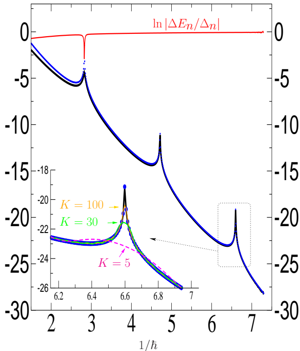
Figure 7: (colour online) For V given by (65) with a = 7/4 and b = 1/2 , we plot \ln |\Delta E_n| (thick black line) for the lowest doublet in the symmetric wells E_n^\pm \simeq \hbar\omega/2 with \omega = 2a\sqrt{2(a^2 - b^2)} \simeq 6.30 . The (blue) dots correspond to estimation (A13) with T = |T|e^{-i\theta} = (K + 1/2)T_m(E_n) - iT_c(E_n) in the limit K \rightarrow \infty ( \theta \rightarrow 0 ). The upper thin (red) curve provides \ln |\Delta E_n/\Delta_n| . The inset provides a magnification of the third spike around 1/\hbar = 6.6 for which T_m(E_n) = 2T_r(E_n) \simeq 1.58 and T_c(E_n) \simeq 1.50 . Here, we have also plotted \ln |\Delta_n(T)| for K = 100 (thin orange, \theta \simeq 0.01 ), K = 30 (thin green \theta \simeq 0.03 ), K = 5 (dashed thin magenta \theta \simeq 0.17 ).
