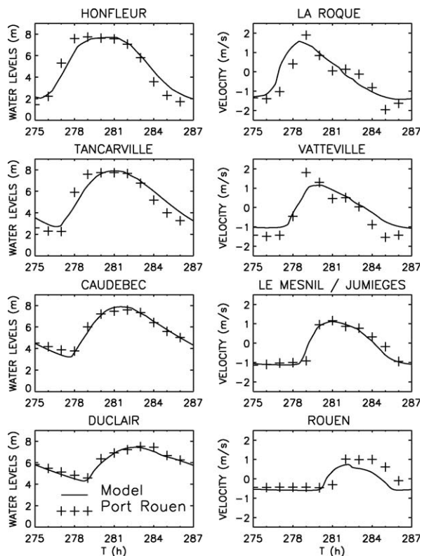
Fig. 3. Calibration results in spring tide: two-phase flow model (—); SHOM (+).
