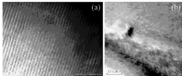
Figure 3: (a) High resolution TEM image of a \text{PrFeAsO}_{1-y} crystal; an undulation of the FeAs layers can be observed. (b) TEM image showing strong contrast, interpreted as an extended point defect.
