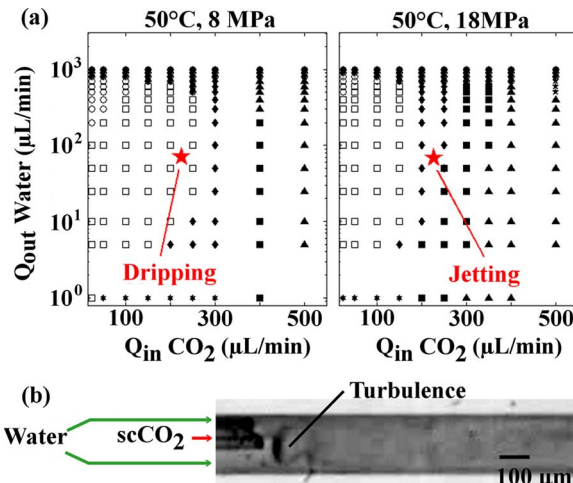
FIG. 3. (Color online) (a) Dynamic phase diagrams in the ( Q_{in} and Q_{out} ) plane of the scCO 2 -liquid water coflowing system, obtained at two different pressures, all other parameters being kept constant ( D=250\ \mu\text{m} , d=75\ \mu\text{m} , and T=50\ ^\circ\text{C} ). (b) Turbulence observed from scCO 2 high flow rate Q_{in}=1000\ \mu\text{L}/\text{min} , in liquid water ( Q_{out}=50\ \mu\text{L}/\text{min} ), for D=250\ \mu\text{m} , d=50\ \mu\text{m} , T=50\ ^\circ\text{C} , and p=8\ \text{MPa} , i.e., for the scCO 2 flow: Re=4500 .
