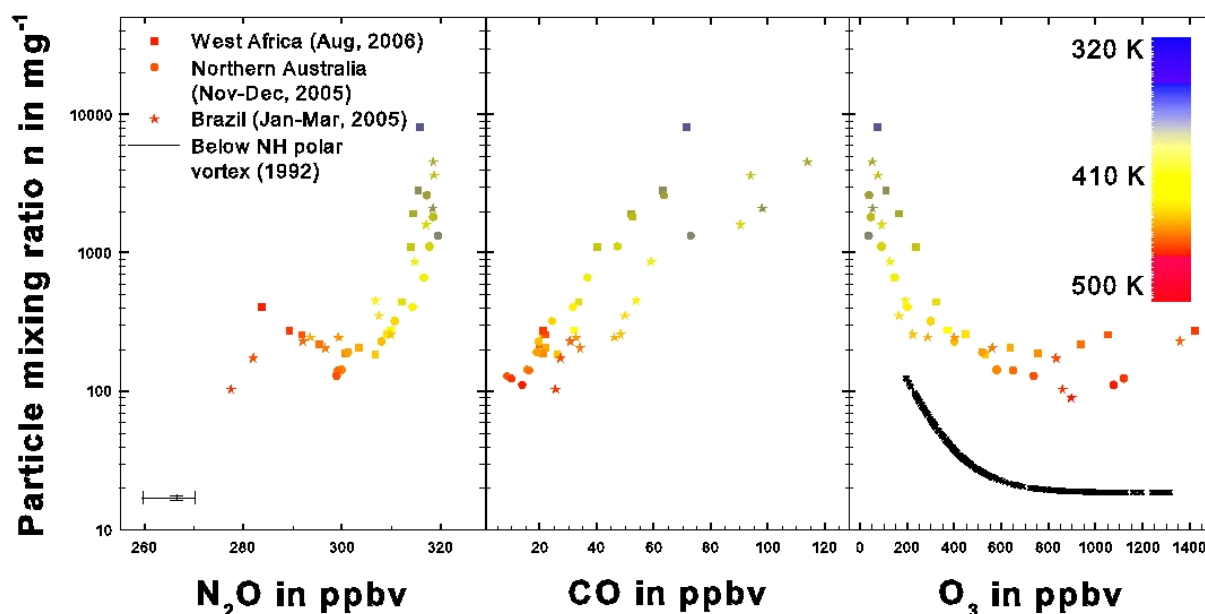
Fig. 8. Correlation of submicron particle mixing ratios n with trace gases \text{N}_2\text{O} , \text{CO} , and ozone for West Africa, Northern Australia, and Brazil. The data points are medians of 10 K potential temperature intervals. The black curve in the right panel is a parameterisation of the 1992 NASA ER-2 data from below the northern hemispheric polar vortex for comparison (see text for details).
