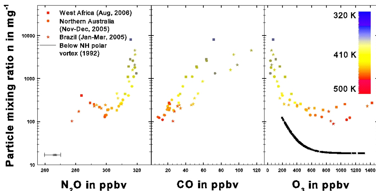
Fig. 8. Correlation of submicron particle mixing ratios n with trace gases \text{N}_2\text{O} , \text{CO} , and ozone for West Africa, Northern Australia, and Brazil. The data points are medians of 10 K potential temperature intervals. The black curve in the right panel is a parameterisation of the 1992 NASA ER-2 data from below the northern hemispheric polar vortex for comparison (see text for details).
