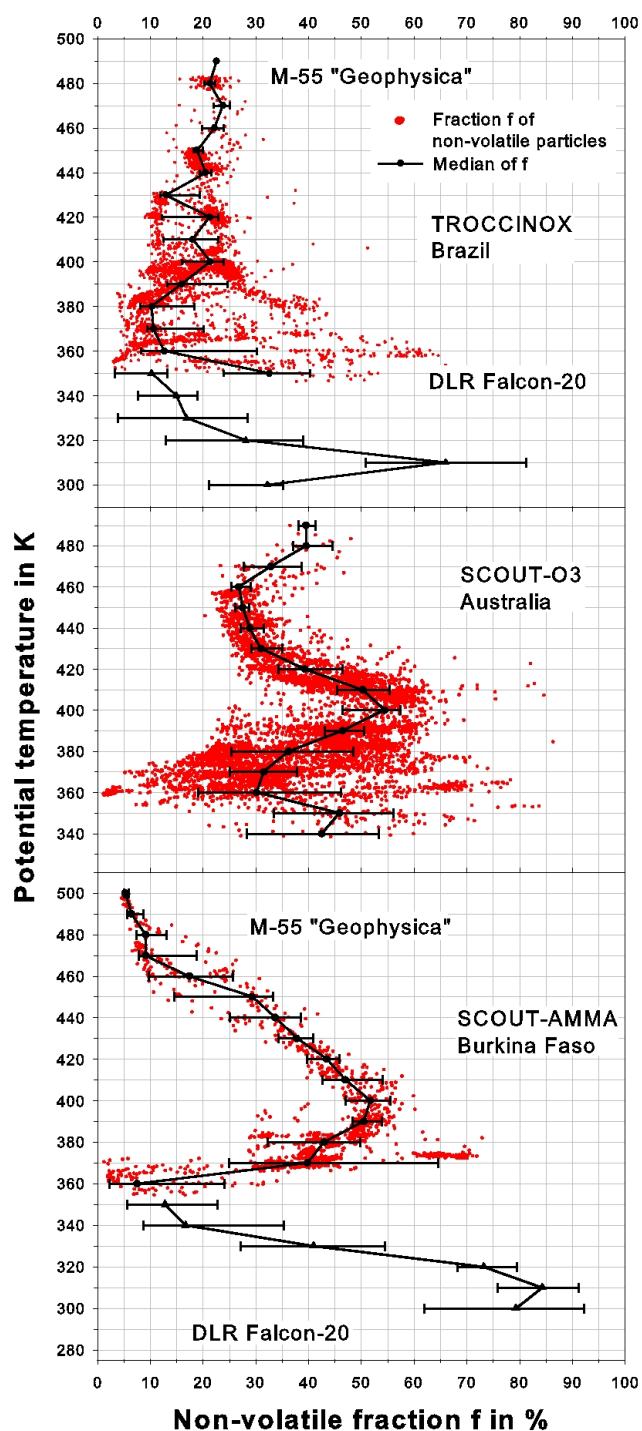
Fig. 11. Ratio f of non-volatile particle number concentration N_{10nv} to total ambient particle number density N_{10} as function of altitude (points: 15 s flight time averages; Symbols: medians, 25% and 75% percentiles of 10 K bins). The data are from the local flights over Araçatuba (Brazil, 2005), Darwin (Australia, 2005), West Africa (red points and line above 360 K). Similarly, thermoenuder measurements of N_7 from the DLR Falcon-20 are included (without individual data points) where available for potential temperature levels below 350 K.
