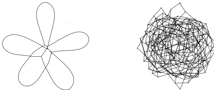
Fig. 1. Two randomly generated subgroups of F(\{a, b\}) depicted by their graphical representation. On the left, a random subgroup for the word-based distribution with 5 words of lengths at most 40. On the right, a random subgroup with 200 vertices for the graph-based distribution. Only the shape of the graph is depicted, edges' labels and directions are not represented. The pictures have been generated by neato . Note that the scale (average distance between two vertices) is not the same on the two pictures. The graphical representation of a subgroup is defined in Section 2.2.
