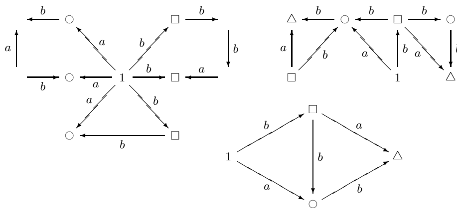
Fig. 2. Some steps of the computation of the Stallings graph for B = \{b^3a^{-1}b^{-1}, aba^{-1}ba^{-1}, b^2a^{-1}\} .
