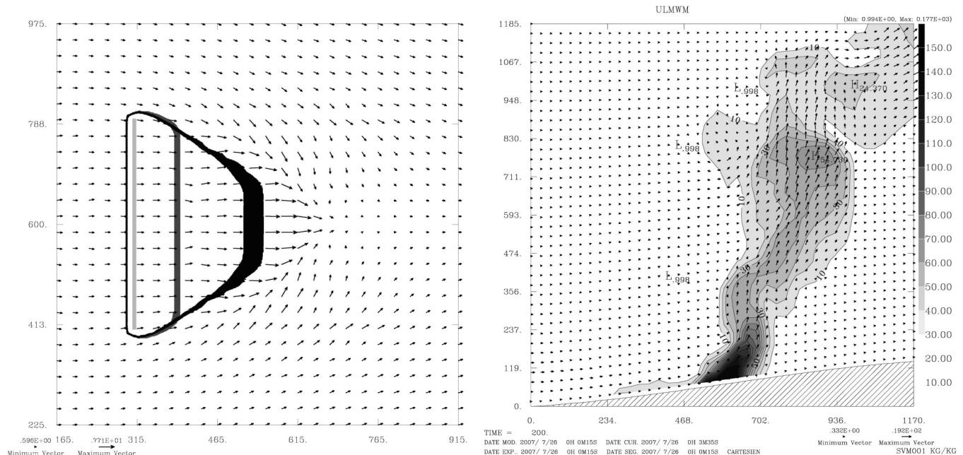
Figure 6. CONF3 (a) Horizontal section (x/y) at Z=10\text{m} , fire line propagation after 200 seconds for the coupled (black) and non-coupled (grey) simulations. Arrows denote the wind vectors of the coupled case. Light-grey line represents the initial ignition for both cases. (b) Cross-section (x/z) of the coupled case at Y=600\text{m} , shading represents concentration of the injected passive tracer.
