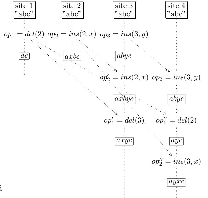
Figure 6. COT Counter-example.
