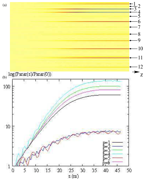
Figure 10: (color online) (a) 2D-Evolution of C(k; z) . Each peak corresponds to a scar mode, denoted here by their order p . (b) Evolution of the intensities of scar modes along the propagation z .
