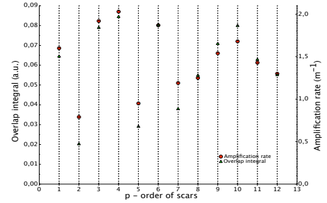
Figure 11: (color online) Comparison of the overlap integral between the intensity of the calculated scar modes and the doped area, and the amplification rates measured in Fig.(10b).
