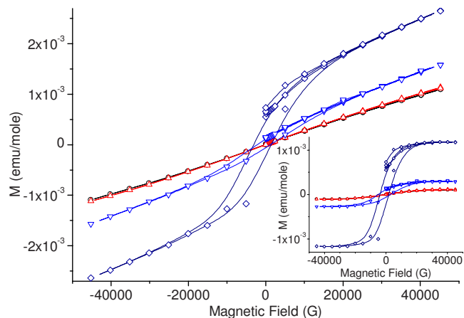
FIG. 3. (Color online) Molar magnetization data vs magnetic field at 5 K for the as-synthesized ( \circ ), Ar-annealed ( \triangle ), 5 h \text{O}_2 -annealed ( \diamond ), and 12 h \text{O}_2 -annealed ( \nabla ) samples. Inset: same data with the linear contribution subtracted ( n_0 : amount of product used for the analysis assuming a zero impurity rate).
