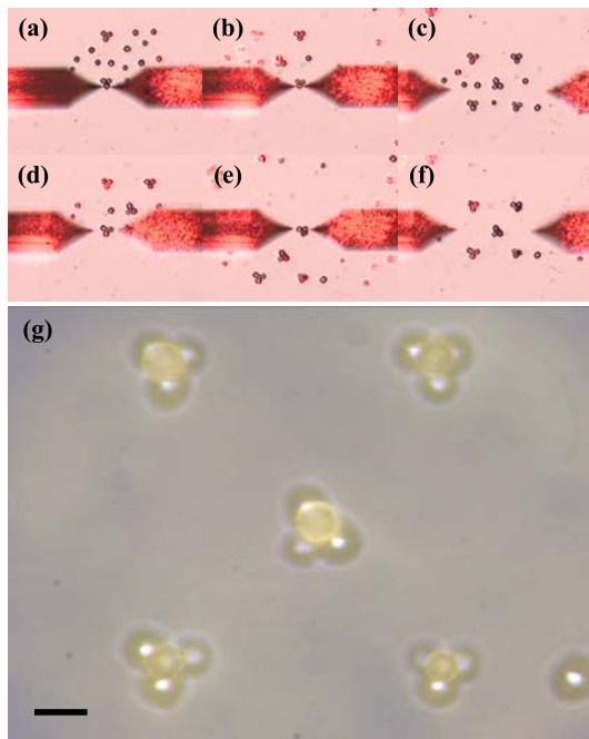
Fig. 6. Assembly results. (a)C(c) show three images intercepted from assembly process of the first layer of the micropylamids. (d)C(f) depict assembly process of the second layer of the micropylamids. The images (a)C(f) are captured under magnification of 20 \mu\text{m} . (g) The 3D microassembly results under magnification of 100\times , in which the scale bar represents 5 \mu\text{m} [31].
