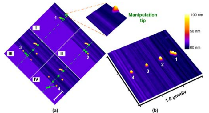
Fig. 8. A parallel imaging/manipulation result with a normal-speed image scan of tip I. (a) Emergences of four particles (with a diameter of 74nm - 82nm) on four different dynamic displays, namely, image I to IV. Once one particle has been fully scanned, a corresponding manipulation task will be activated to push it to its destination. (b) A manipulation result. Four nanoparticles were pushed along a line within the frame period of the image scan. The total manipulation time for these four particles was less than one minute, which is much less than the entire imaging time of ten minutes [33].
