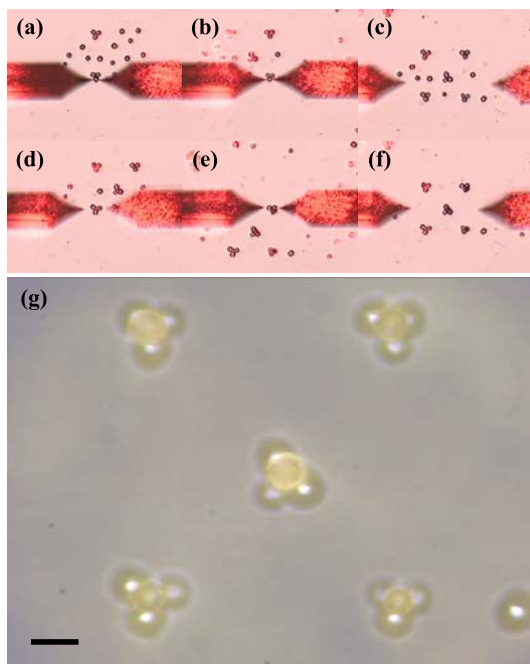
Fig. 6. Assembly results. (a)C(c) show three images intercepted from assembly process of the first layer of the micropylramids. (d)C(f) depict assembly process of the second layer of the micropylramids. The images (a)C(f) are captured under magnification of 20 \mu\text{m} . (g) The 3D microassembly results under magnification of 100\times , in which the scale bar represents 5 \mu\text{m} [31].
