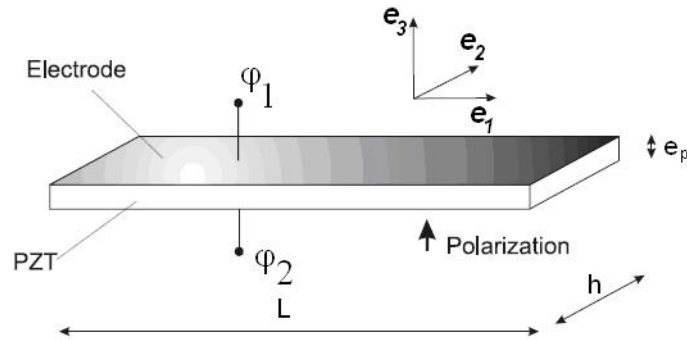
Figure 3: Thickness-polarized piezoelectric beam transducer with electroded surfaces, and orientation in the material reference frame ( \mathbf{e}_1, \mathbf{e}_2, \mathbf{e}_3 ). \varphi_1 and \varphi_2 denotes the electric potential of the electrodes.
