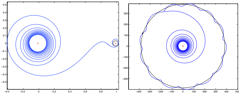
Fig. 6. Focal point computation, \varepsilon = 2.440e - 1 . The target is a lunar orbit, and the focal point test ensures local optimality of the trajectory. The leftmost frame is the rotating frame, the rightmost one is fixed.
