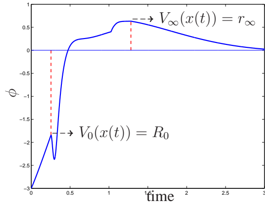
Fig. 2. Time-evolution of the uniting controller \phi .
