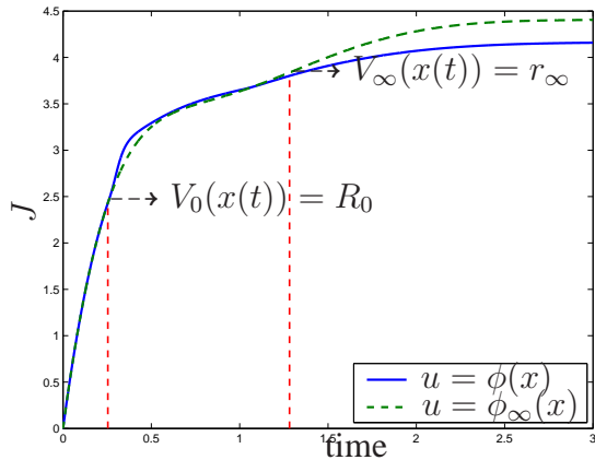
Fig. 1. Time-evolution of the cost function J with the controls \phi (in plain line) and \phi_\infty (in dashed line).
