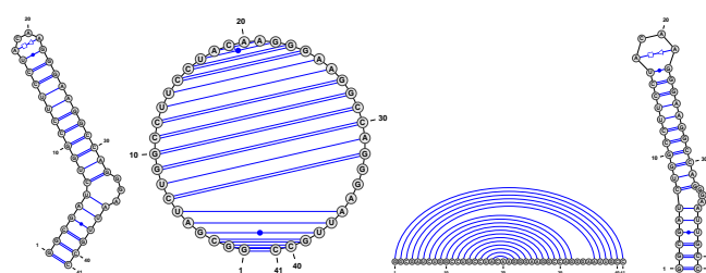
Fig. 1. Four representations ( Radial , Circular , Linear and NView ) of the GAG-Pol -1 frameshift-inducing element in HIV-1 (PDBID:1ZC5) as rendered by VARNA under default settings.
