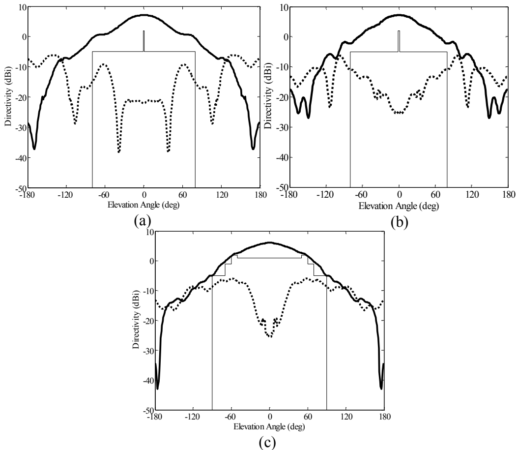
Figure 2. The measured radiation patterns (RHCP : — ; LHCP : ... ; Minimum required RHCP : - - -) for the multi-band antenna at: (a) 1.197 GHz, (b) 1.575 GHz and (c) 2.245 GHz
