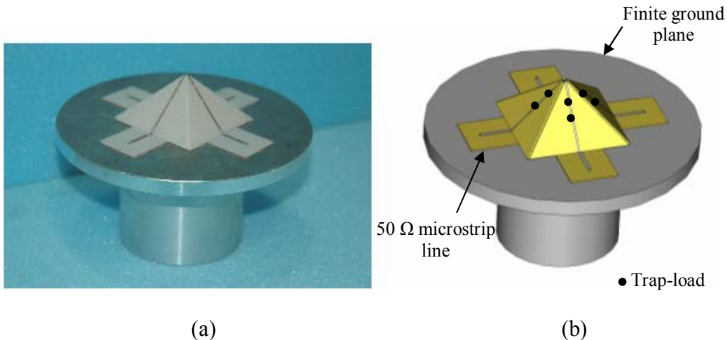
Figure 1. Pyramidal triple-frequency trap loaded antenna: (a) the practical realization and (b) the simulated model
