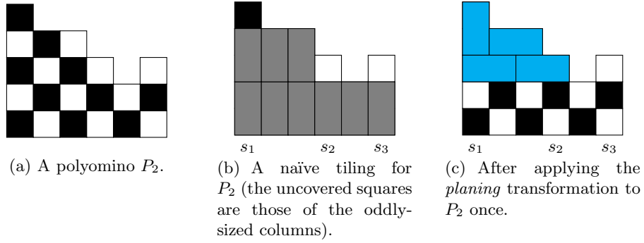
Fig. 4. Tilings of P_2 , which has three oddly-sized columns.
