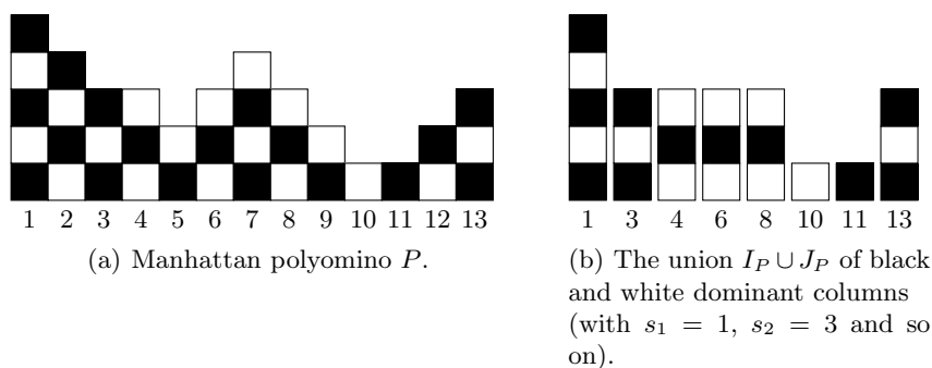
Fig. 2. Construction of a \{s_1, \dots, s_n\} set.
