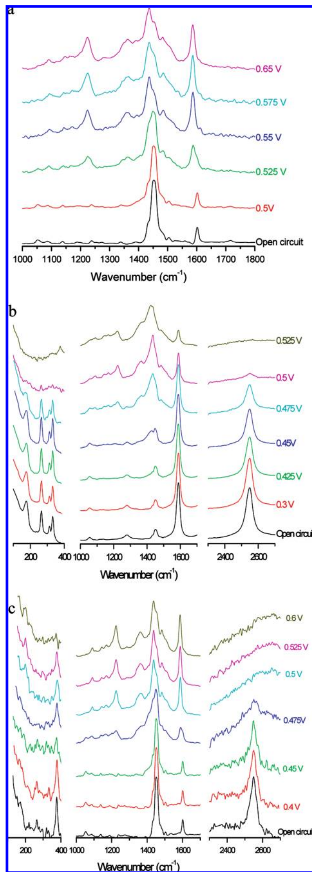
Figure 5. Raman spectra recorded for increasing working electrode potentials ( \lambda_{\text{exc}} = 1064 nm; electrolyte \text{Bu}_4\text{NBF}_4/\text{acetonitrile} ; reference electrode \text{Ag}/\text{Ag}^+ ). (a) Thin layer of QTF12 deposited on platinum electrode; (b) thin layer of QTF12-1.0%DWCNT deposited on platinum electrode; (c) thin layer of QTF12-0.1%DWCNT deposited on platinum electrode.
